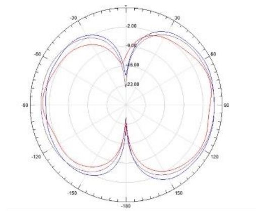
Figure 7: Radiation Pattern
